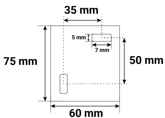
Fixing diagram
