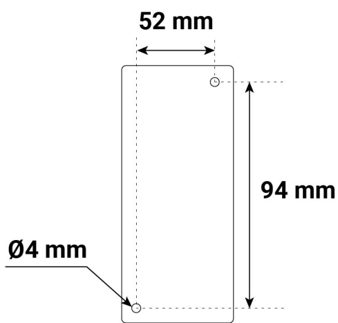
Fixing diagram
