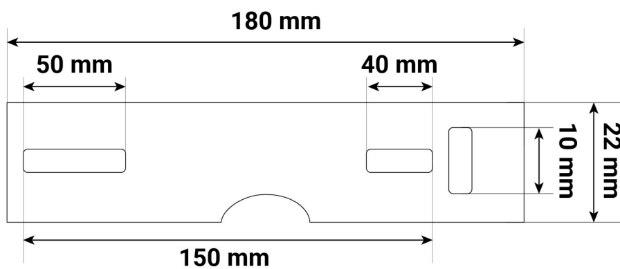
Fixing diagram
