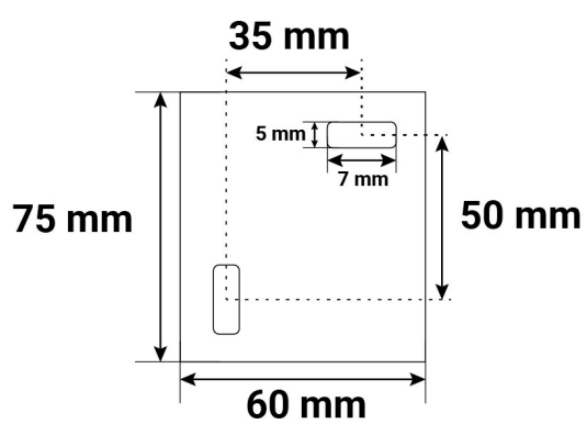
Fixing diagram
