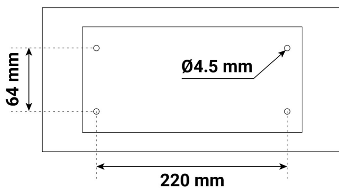
Fixing diagram
