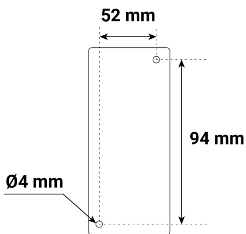
Fixing diagram
