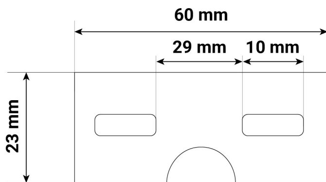
Fixing diagram
